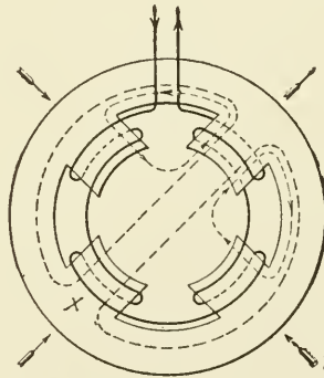
Fig. 134. Magnetic Field of Motor When One Field Coil is Reversed
